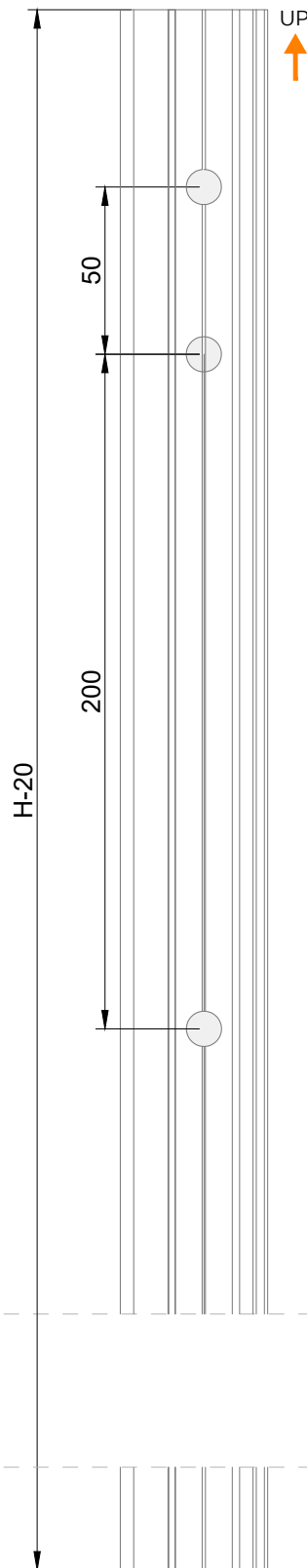
VE50FLM
