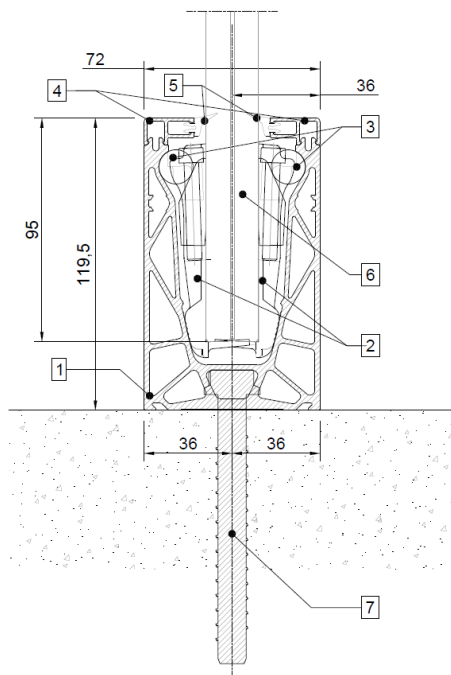
Figure 3 – Scheme of the DEFENDER system DF810LM21
