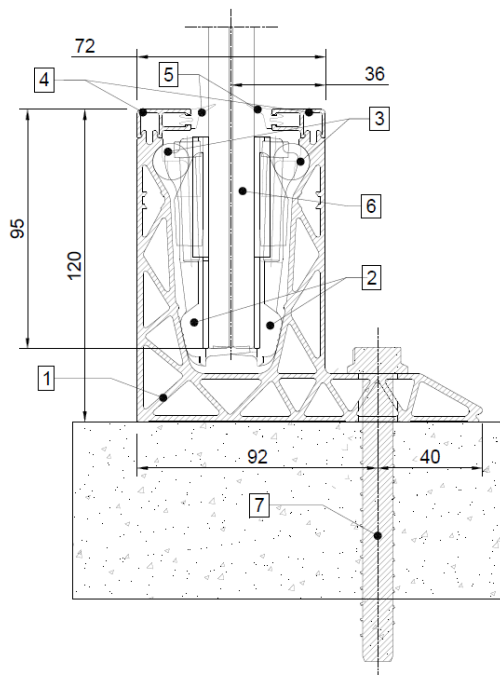
Figure 5 – Scheme of the DEFENDER system DF810DK17
