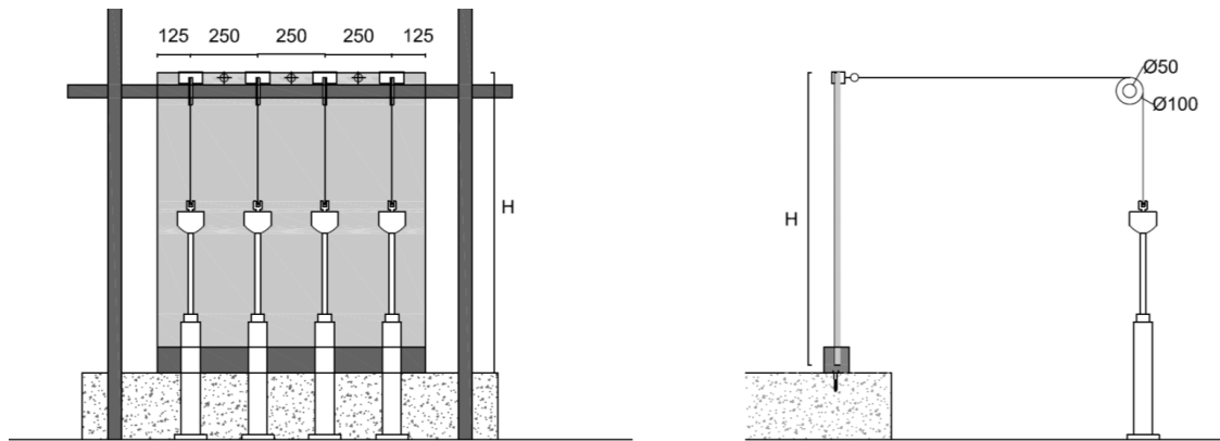
Figure 1 - scheme of the test setup
