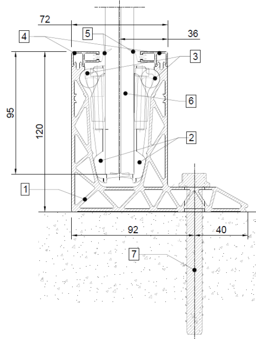
Figure 6 – Scheme of the DEFENDER system DF810DK21
