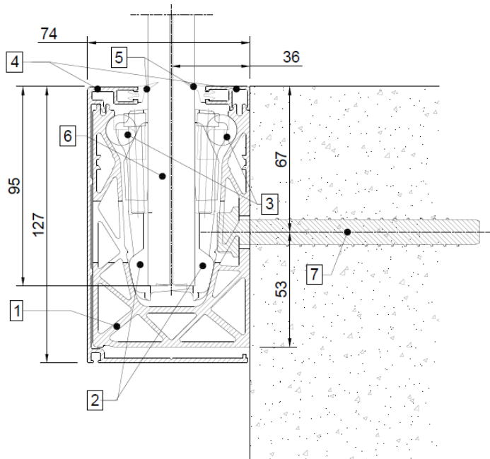
Figure 5 – Scheme of the DEFENDER system DF810FR21
