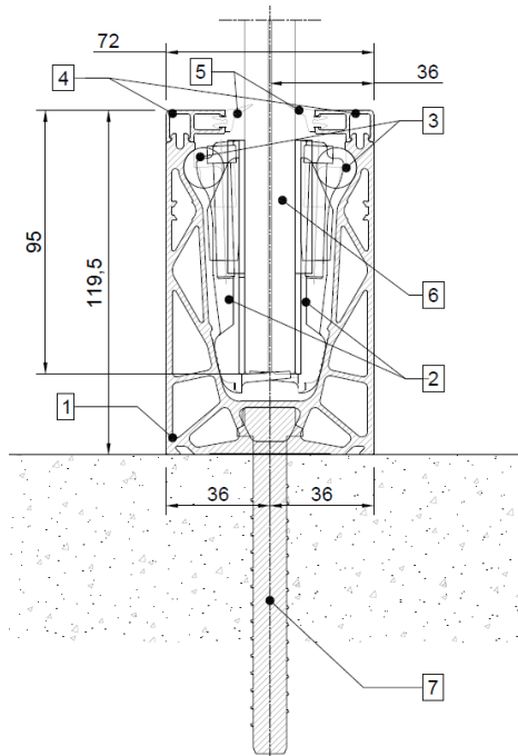
Figure 2 – Scheme of the DEFENDER system DF810LM17
