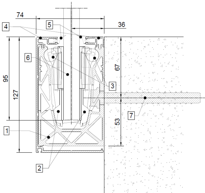
Figure 4 – Scheme of the DEFENDER system DF810FR17
