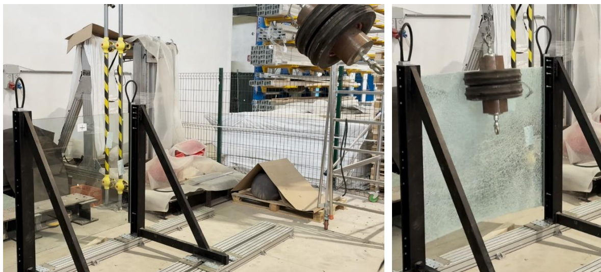
Impact test 1 with semi-rigid body: h 700 mm (T1)
