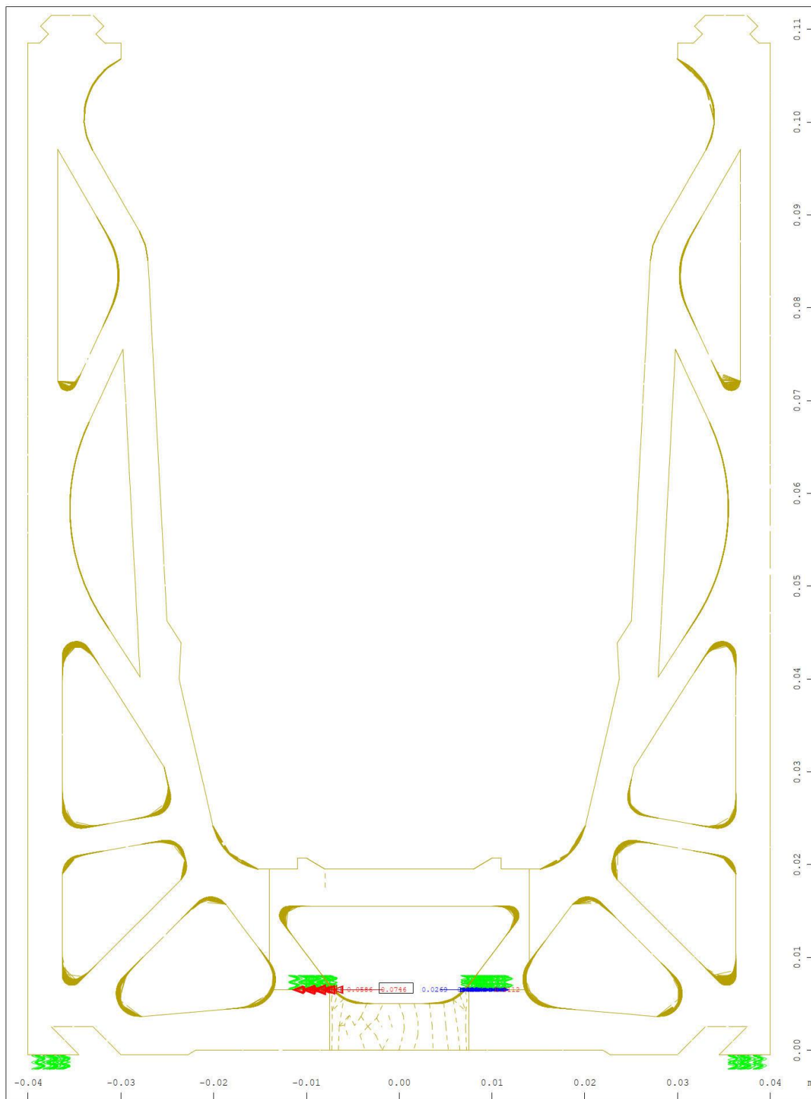
Y Sector of system Group 2 10 11 20 M 10 : 4.88 X Supporting springs , Spring force in global X, nonlinear Loadcase 10 ULS , 1 cm 3D = 0.0500 kN (Min=-0.0746) (Max=0.0287) (total: -0.900)
