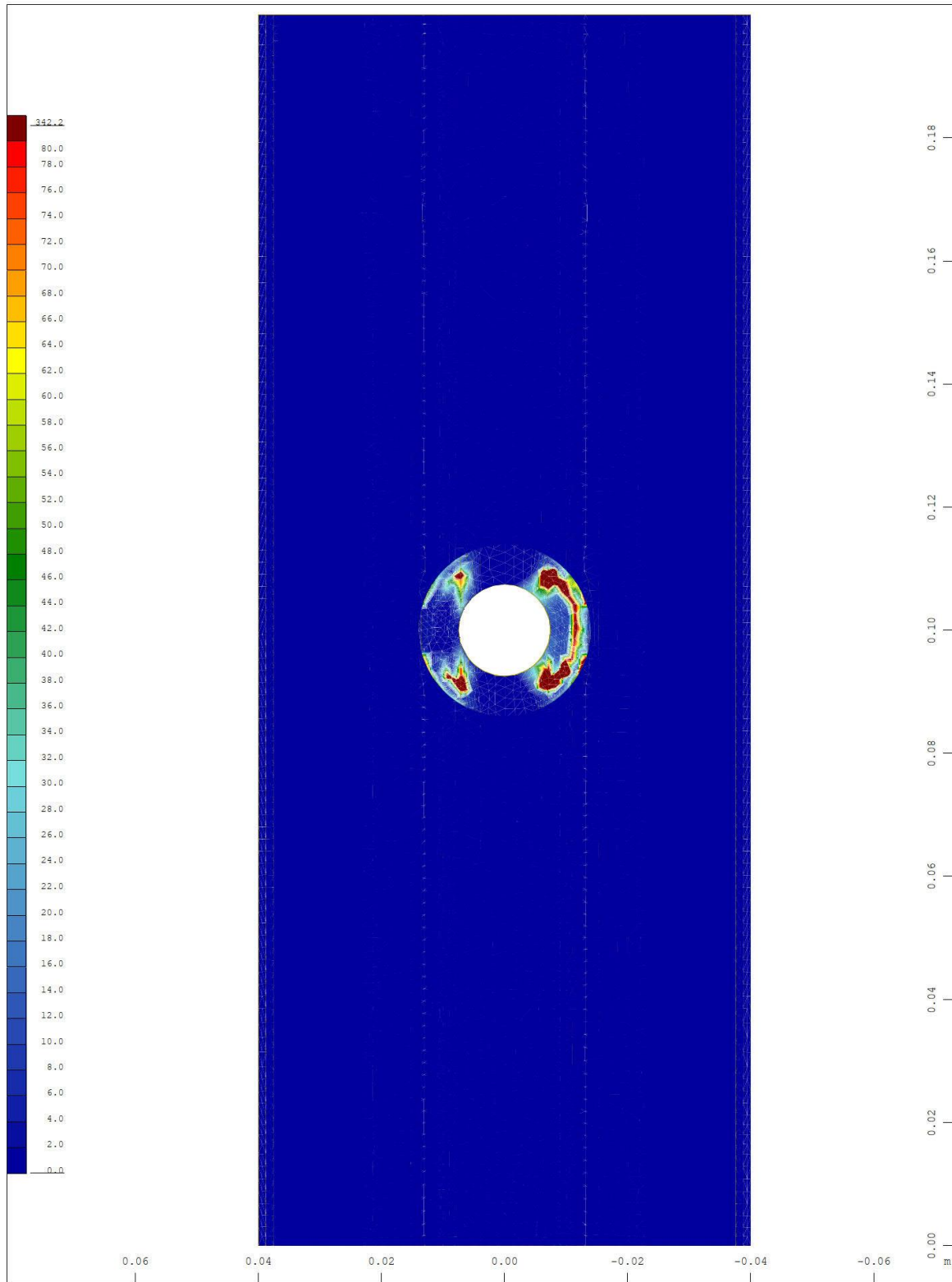
Sector of system Group 2 Plastic deviatoric strain \leftrightarrow , nonlinear Loadcase 10 ULS, Material law Mat.type 17 , BRIC Gauss points in Node o/oo, from 0 to 80.0 step 2.00 M 10 : 8.60
