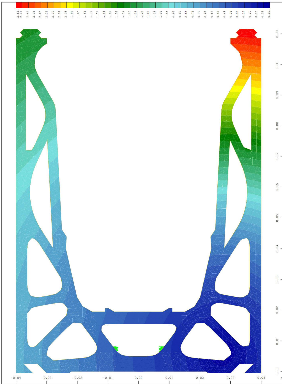
Y Sector of system Group 2 20 M 10 : 5.15 Z-X Nodal displacement vector in Node, nonlinear Loadcase 10 ULS , from 0.0166 to 2.55 step 0.0635 mm
