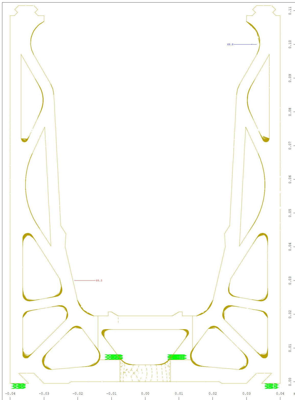
Y Sector of system Group 2 10 11 20 M 10 : 4.88 X All loads, nonlinear Loadcase 10 ULS , (1 cm 3D = unit) Free line load (force) in global X (Unit=50.0 kN/m (Min=-64.3) (Max=68.8))
