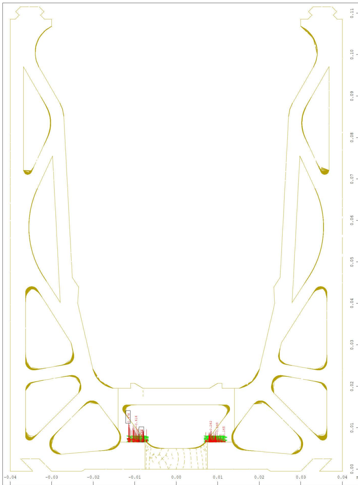
Y Sector of system Group 2 20 X Supporting springs , Spring force in global Y, nonlinear Loadcase 10 ULS , 1 cm 3D = 0.500 kN (Min=-0.478) (Max=0) (total: -25.5)
