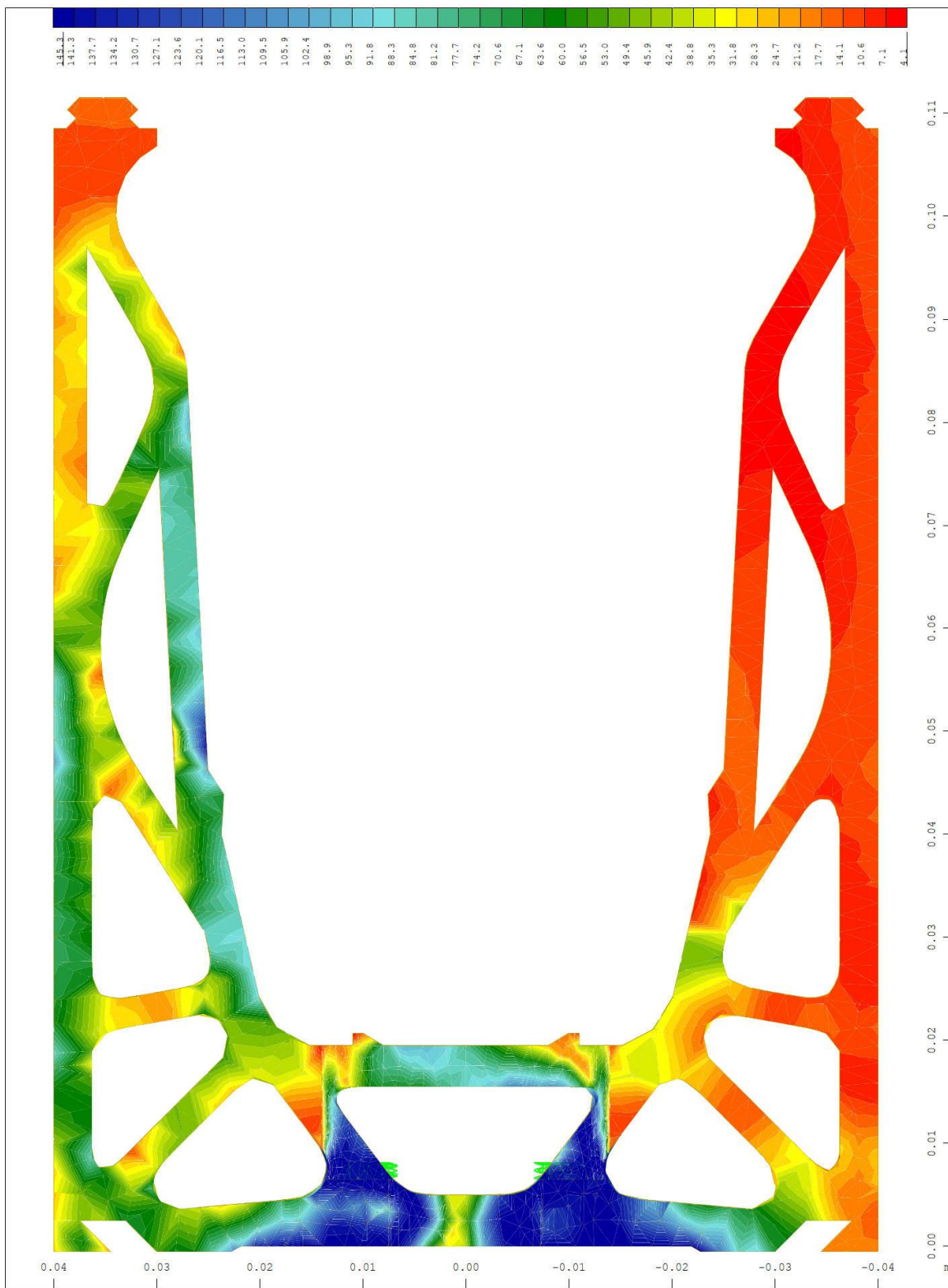
Sector of system Group 2 20 v.Mises stress from middle of element \leftrightarrow , nonlinear Loadcase 10 ULS , from 4.08 to 145.3 step 3.53 MPa M 10 : 5.15
